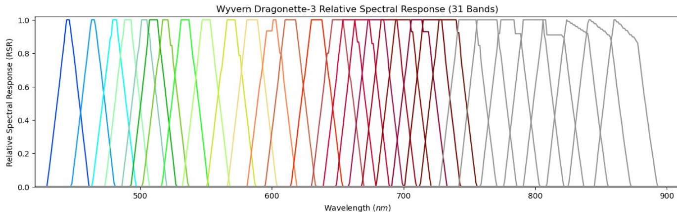
Relative spectral response for the Dragonette-3 satellite
