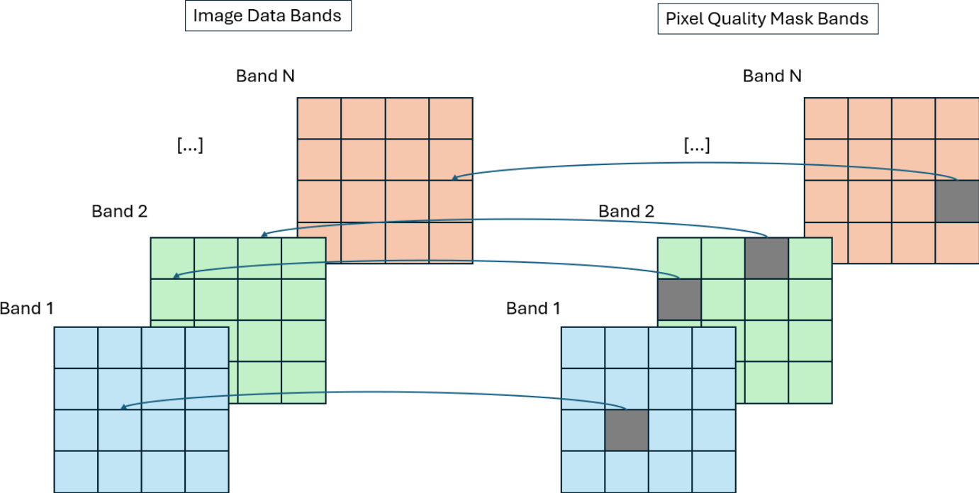
Relationship between bands and pixels in the pixel quality mask raster and the image data raster
