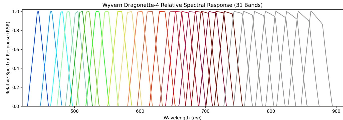
Relative spectral response for the Dragonette-4 satellite
