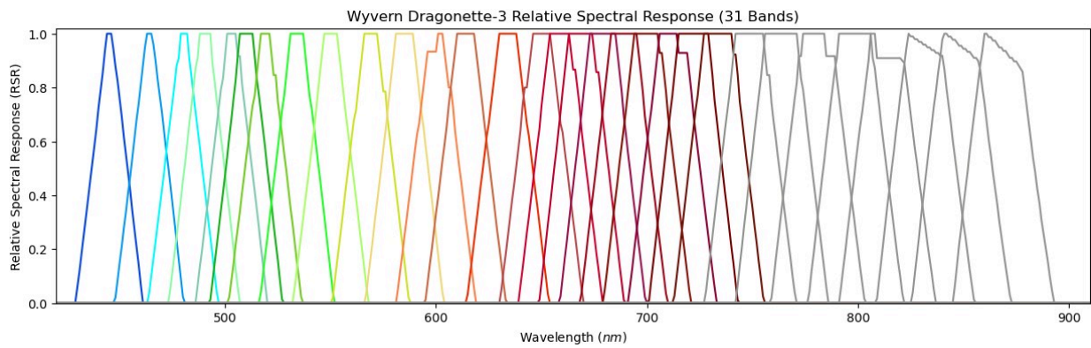
Relative spectral response for the Dragonette-3 satellite
